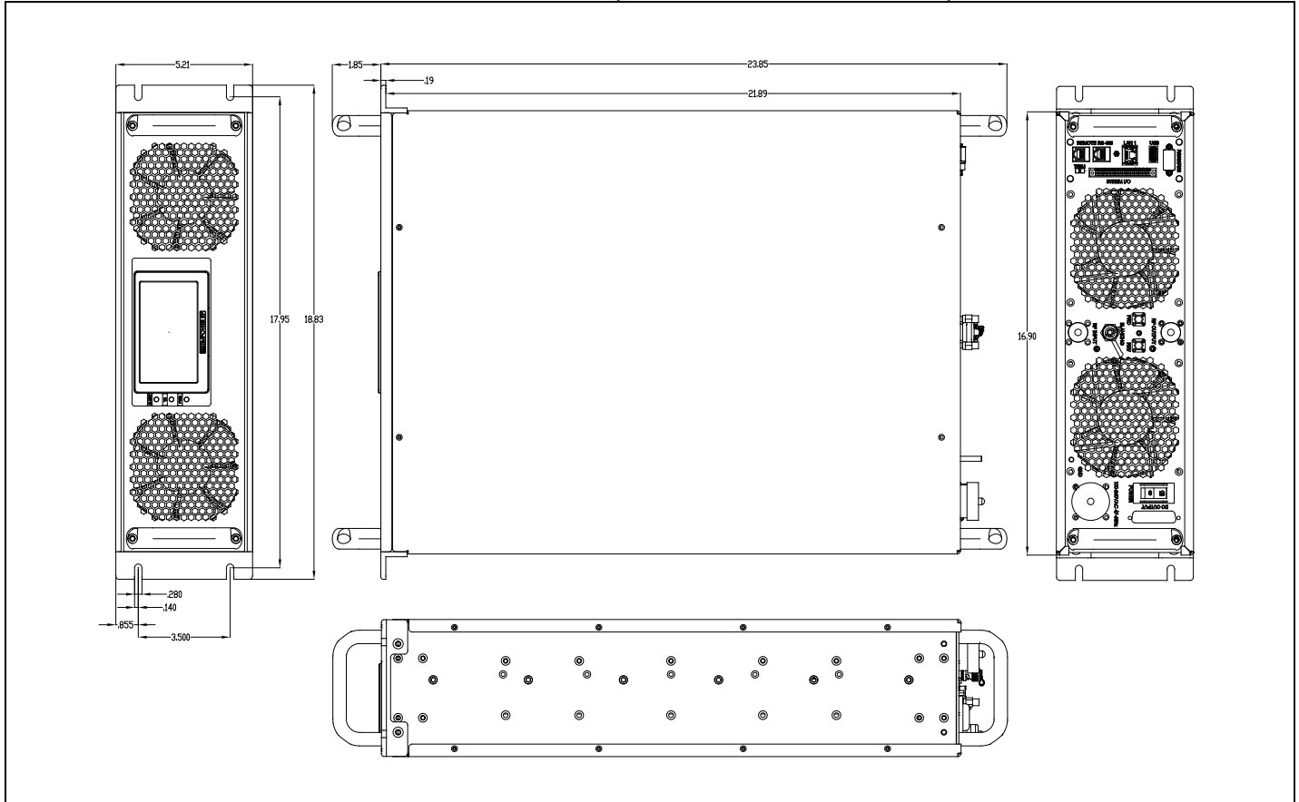
MECHANICAL OUTLINE - (Shown with rear RF connectors)
